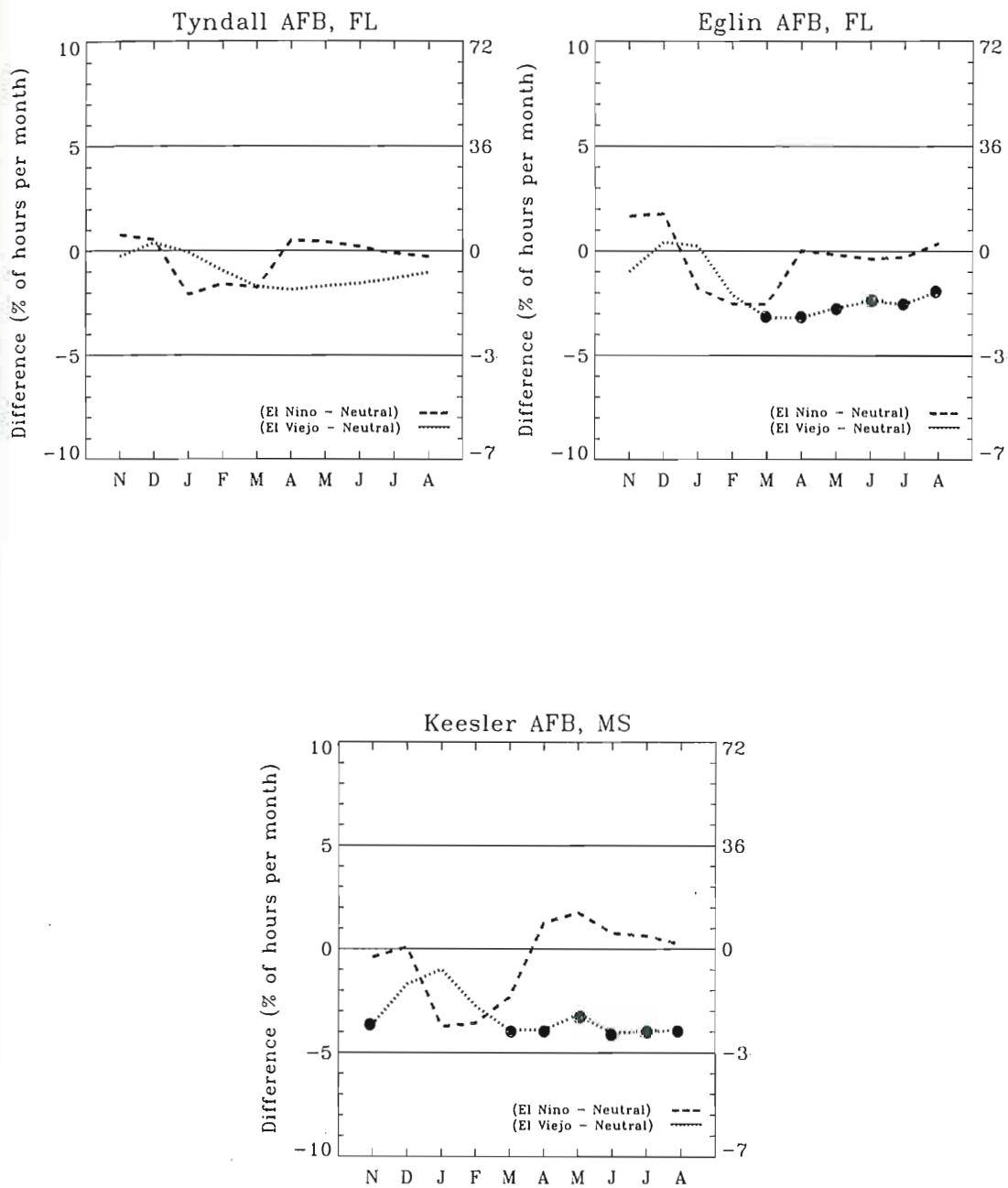
FIG. 10. Difference of means based on resampled data for fog at Tyndall AFB, FL, Eglin AFB, FL, and Keesler AFB, MS. Center month of three month season along abscissa. Percentage difference along left ordinate axis. Approximate hourly difference along right ordinate axis. Dots mark the seasons with a significant difference based on a two tailed T-test using \alpha = 0.05
