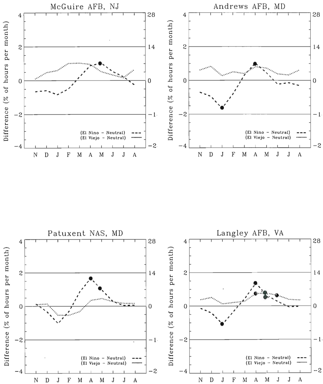
FIG. 15. Difference of means based on resampled data for IFR conditions at McGuire AFB, NJ, Andrews AFB, MD, Patuxent NAS, MD, Langley AFB, VA. Center month of three month season along abscissa. Percentage difference along left ordinate axis. Approximate hourly difference along right ordinate axis. Dots mark the seasons with a significant difference based on a two tailed T-test using \alpha = 0.05
