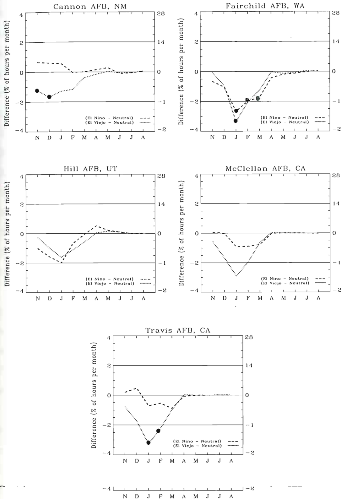
FIG. 16. Difference of means based on resampled data for IFR conditions at Cannon AFB, NM, Fairchild AFB, WA, Hill AFB, UT, McClellan AFB, CA, and Travis AFB, CA. (See Fig. 15)
