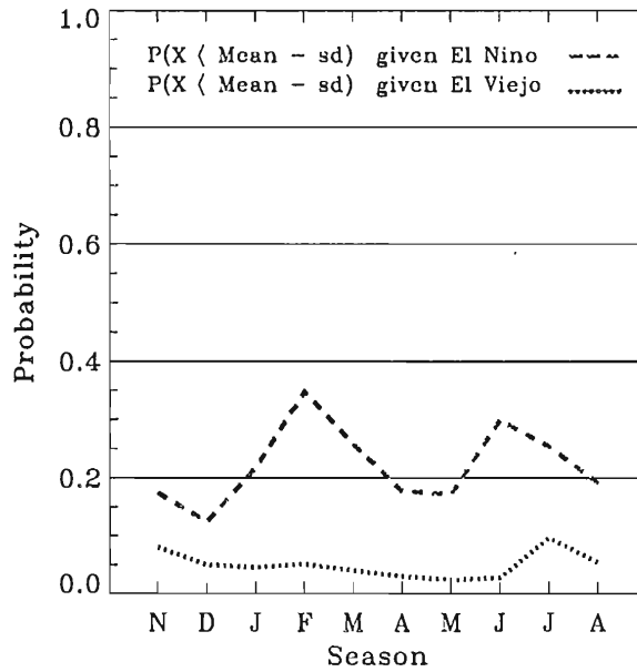
FIG. 14. Conditional probabilities based on resampled data for occurrence of IFR conditions at Dobbins ARB, GA.
