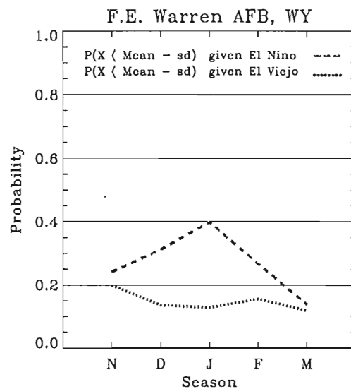
FIG. 20. Conditional probabilities based on resampled data for occurrences of snow at Cannon AFB, NM and F.E. Warren AFB, WY.
